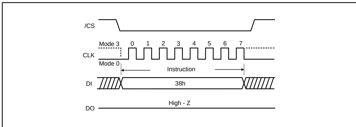
Figure 51. Enter QPI Instruction (SPI Mode only)
