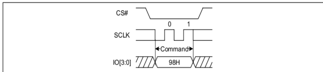
Figure 44d Global Block/Sector Unlock Sequence Diagram (QPI)
