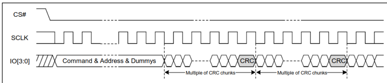
Figure 4. CRC Timing
