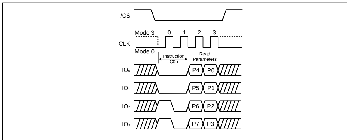
Figure 50. Set Read Parameters Instruction (QPI Mode only)
