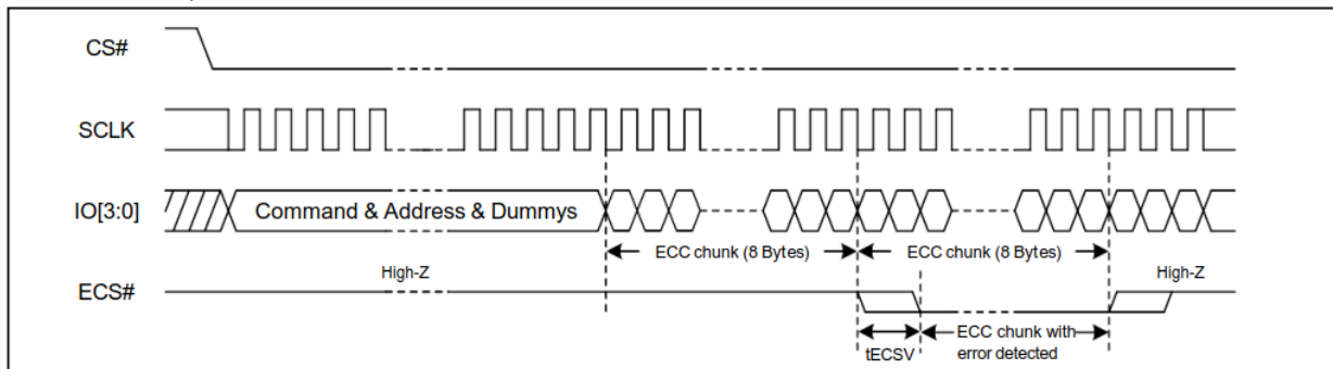
Figure 3. ECS# Timing
