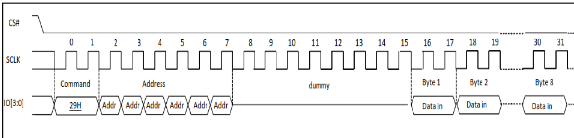
Figure 47b Unlock Password Sequence Diagram (QPI)
