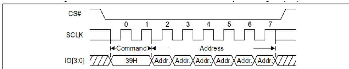
Figure 43d Individual Block/Sector Unlock command Sequence Diagram (QPI)
