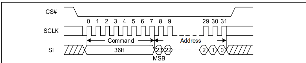
Figure 43a Individual Block/Sector Lock command Sequence Diagram (SPI)
